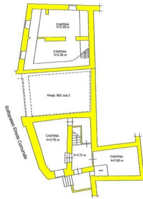
PIANO TERRA
