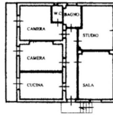
PIANO TERRA H = 3.00
