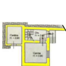
PIANO SEMINTERRATO
