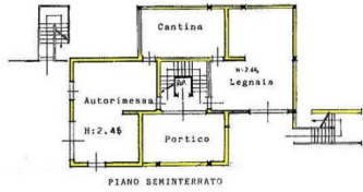
PIANO SEMINTERRATO
