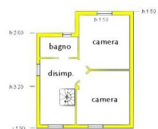
PIANTA PIANO MANSARDA
