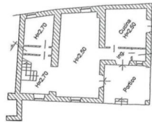
PIANO TERRA
